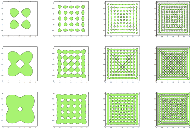
Fig. 1. \Omega = (0, \pi)^2 . Row 1: L = 0.2 ; row 2: L = 0.4 ; row 3: L = 0.6 . From left to right: N = 2 (4 eigenmodes), N = 5 (25 eigenmodes), N = 10 (100 eigenmodes), N = 20 (400 eigenmodes). The optimal domain is in green.
