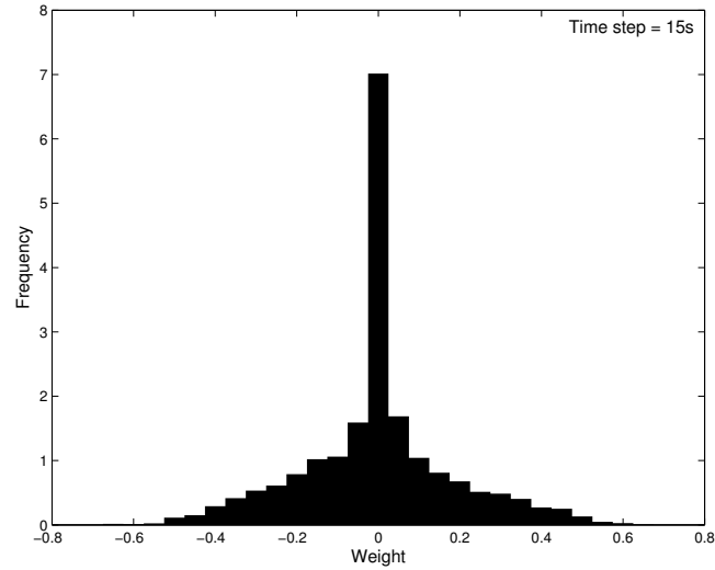
Figure 9: Distribution of weights considering the unitarian Euclidean norm. The mass around zero is important but yet the distribution suggests the dynamics is actively participated by a large portion of the considered stocks. The depicted case corresponds to a time scale of 15s; the remaining ones keep qualitatively the same look.
